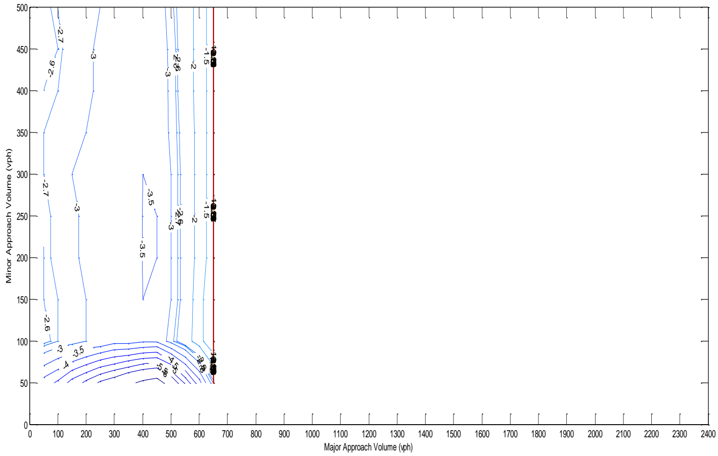
Figure A.166 Contour plot at BF=0.5, LTP=10%, TP=2%
