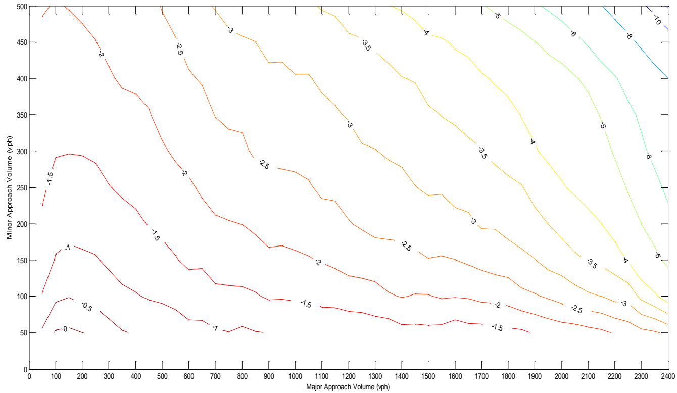
Figure 5.15 Contour plot for total intersection delay difference between CFI and standard signalized intersection at BF=0.7 ,
