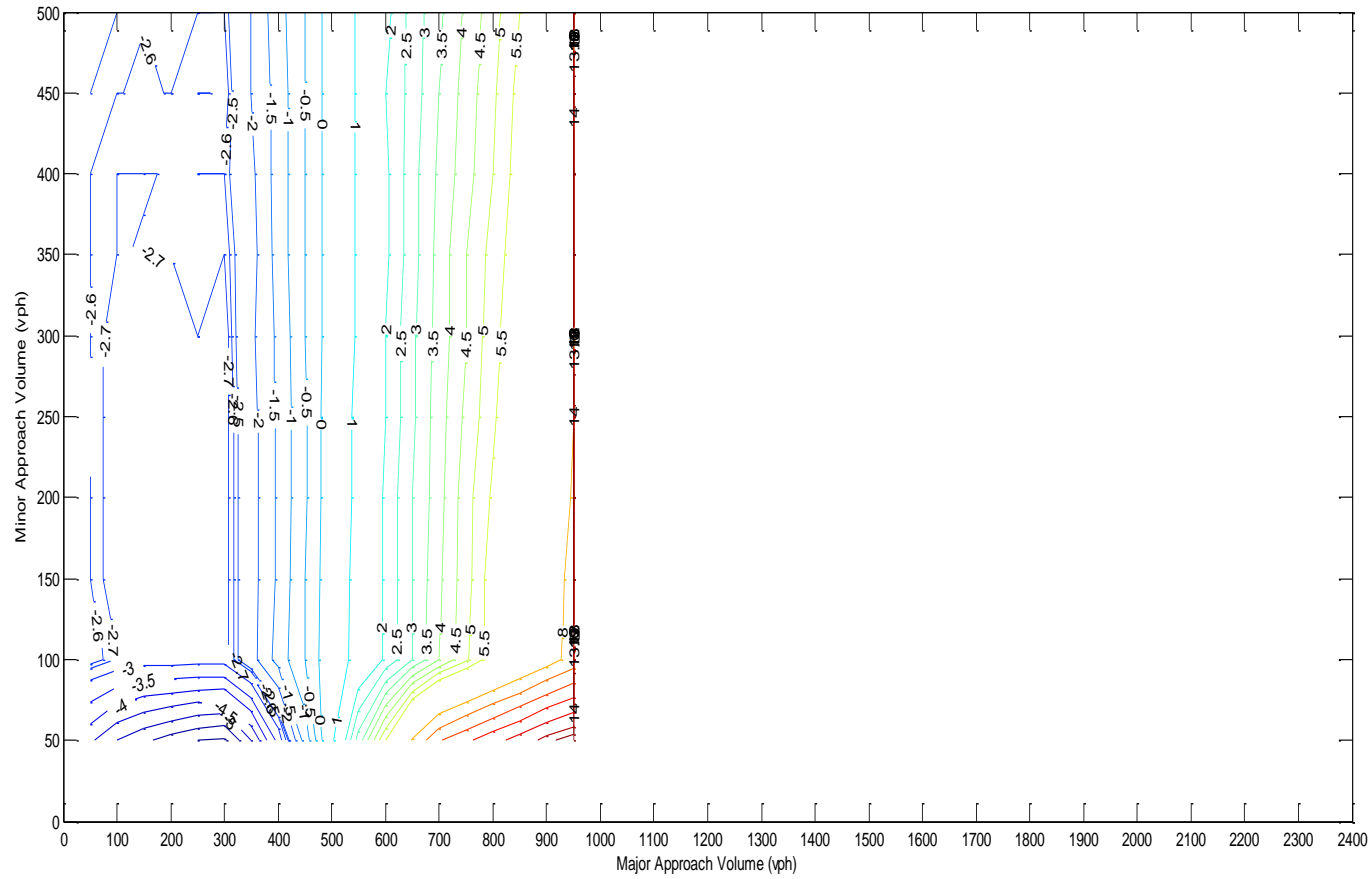
Figure A.183 Contour plot at BF=0.7, LTP=5 %, TP=5 %
