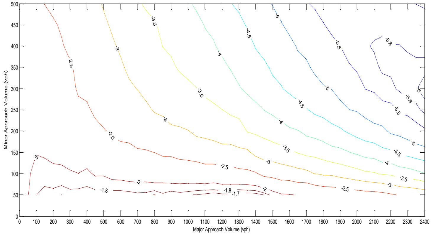
Figure A.149 Contour plot at BF=0.6, LTP=10 %, TP=5 %
