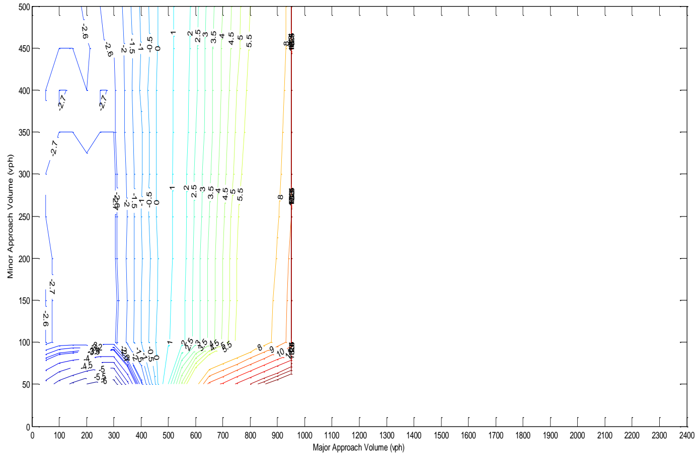
Figure A.192 Contour plot at BF=0.7, LTP=5 %, TP=10 %
