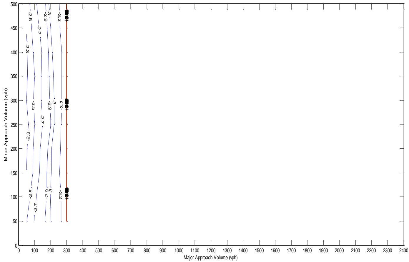
Figure A.207 Contour plot at BF=0.7, LTP=15%, TP=2%
