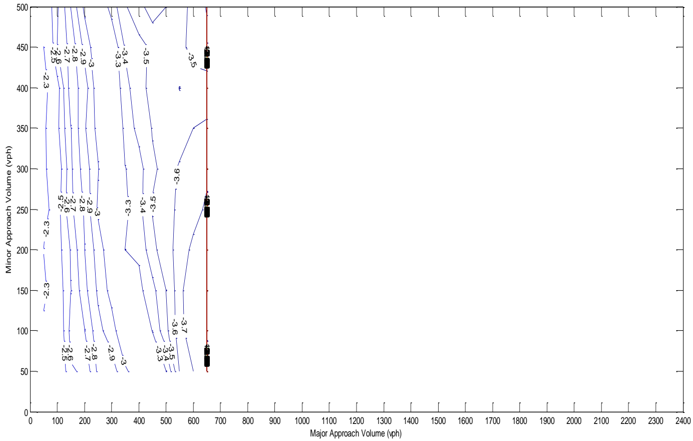
Figure A.202 Contour plot at BF=0.5, LTP=10%, TP=2%
