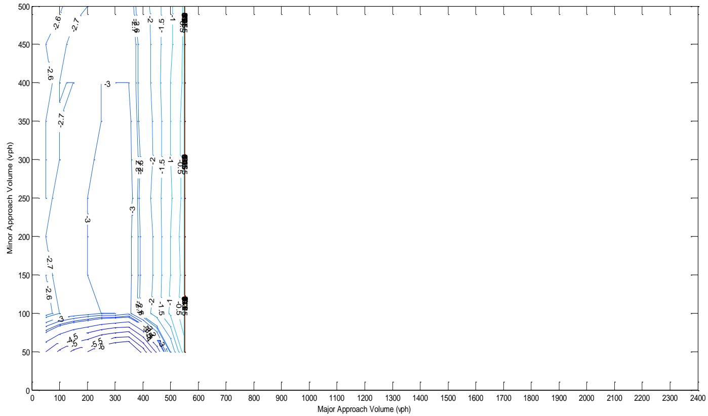
Figure A.194 Contour plot at BF=0.6, LTP=10 %, TP=10 %
