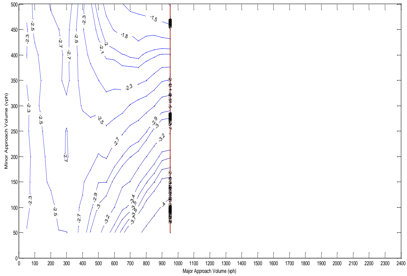
Figure A.210 Contour plot at BF=0.7, LTP=5%, TP=5%
