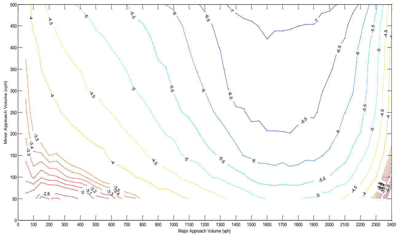
Figure A.58 Contour plot at BF=0.5, LTP=10%, TP=2%
