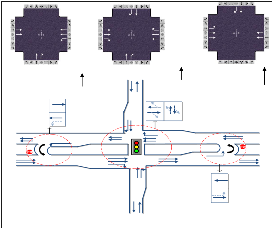
Figure 4.2 Equivalent phases and lane configuration of MUT considered in network coding in HCS 2010 ® Streets
