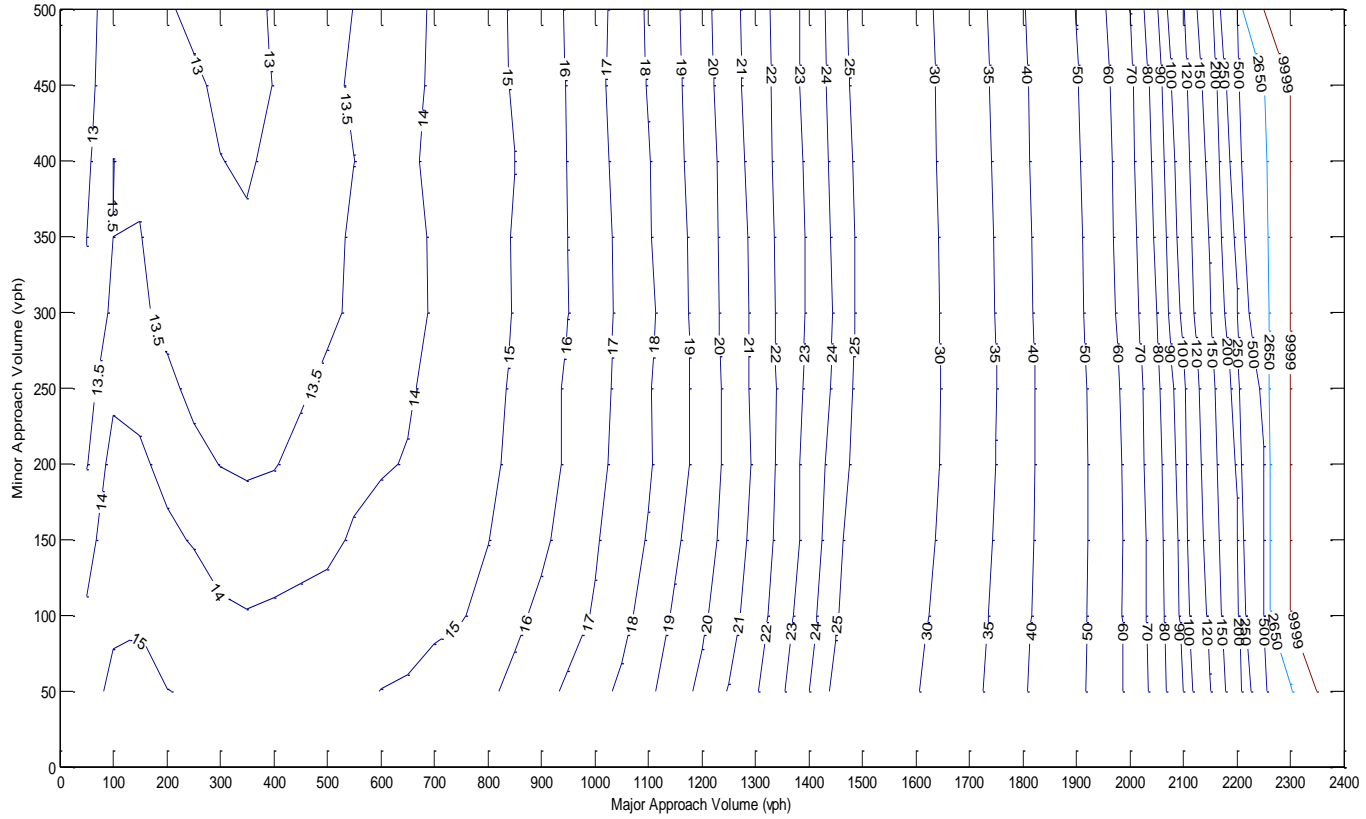
Figure A.35 Contour plot at BF=0.6, LTP=15%, TP=2%
