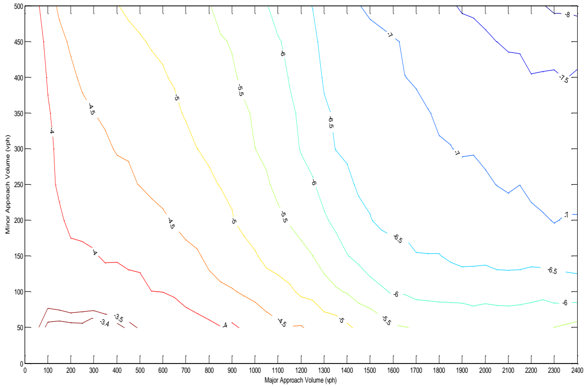
Figure A.64 Contour plot at BF=0.5, LTP=5 %, TP=5 %
